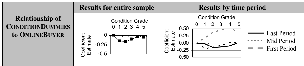
Figure 6: Plots of the coefficients for the CONDITIONDUMMIES in the OnlineBuyer model.
