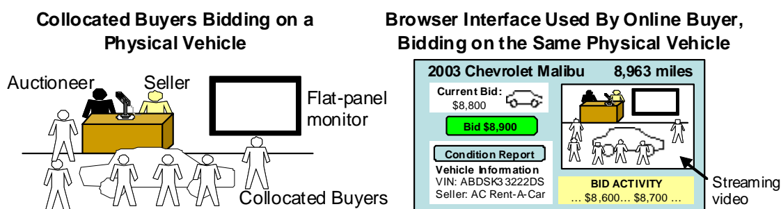
Figure 1: The collocated and online buyer participation channels for physical vehicles.
