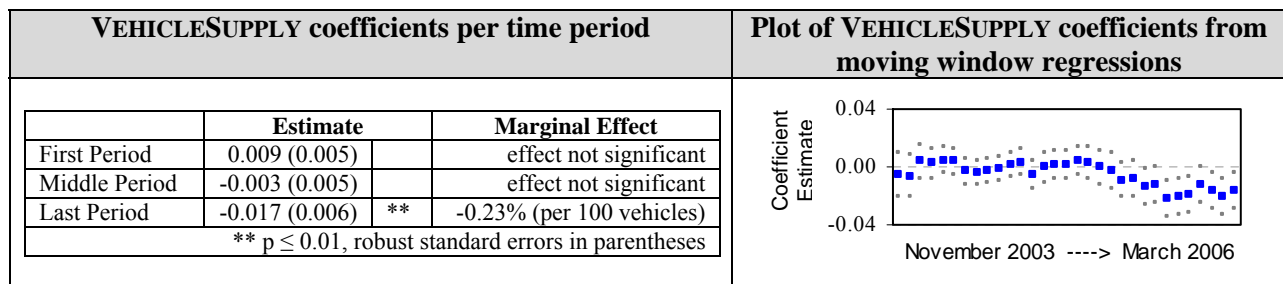
Figure 7: Examination over time of the VEHICLESUPPLY coefficient in the OnlineBuyer model.
