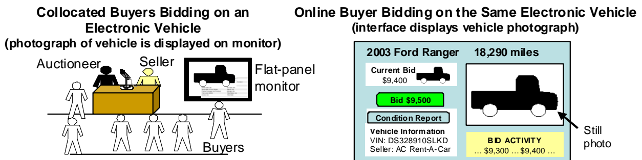
Figure 2: The physical and electronic buyer participation channels for electronic vehicles.
