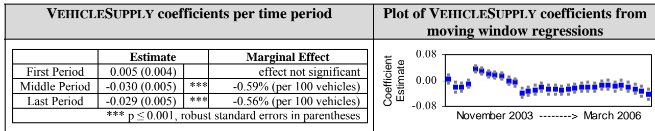
Figure 4: Examination over time of the VEHICLESUPPLY coefficient in the ElectronicVehicle model.
